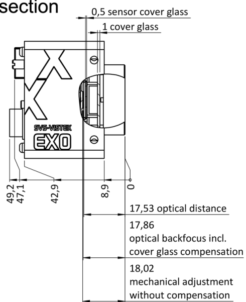
right side
