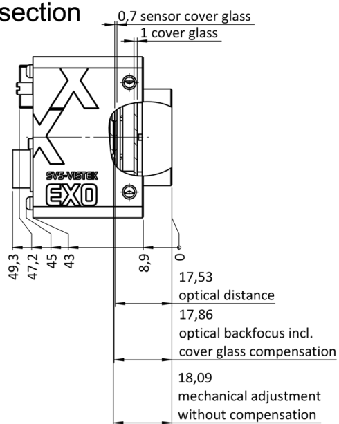
right side
