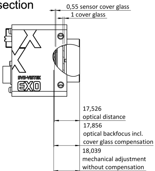
right side
