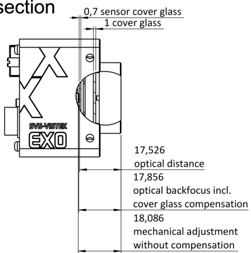
right side
