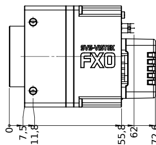
right view
