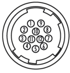
Hirose 12 Pin
