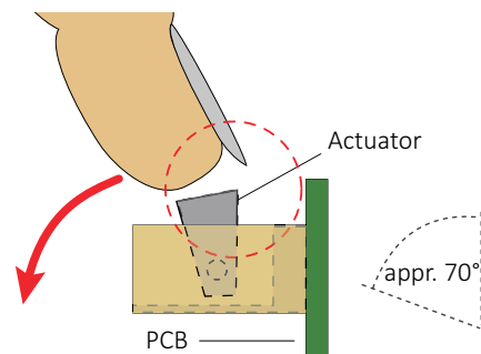
Figure 26: Opening the FPC connector
