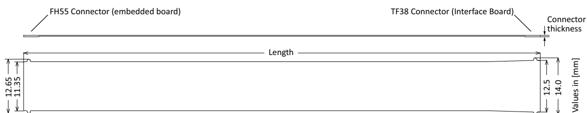
Figure 9: Alvium CSI-2 Flex: FPC Cable: Technical drawing
