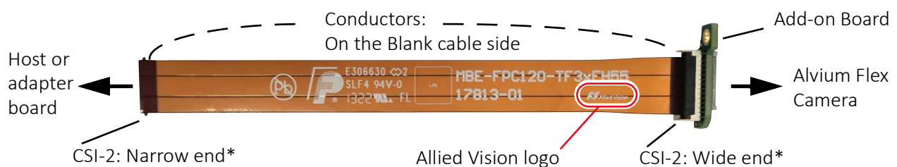
Figure 20: Correct orientation of FPC cables
