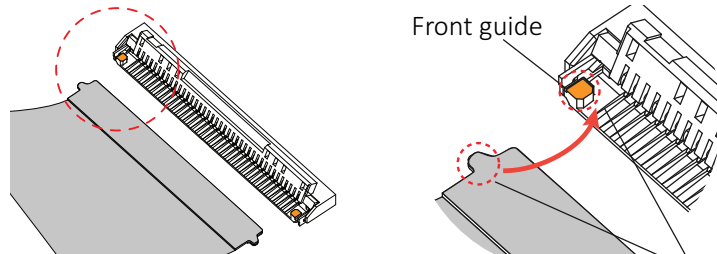
Figure 21: FPC cable and FPC connector (open position)
