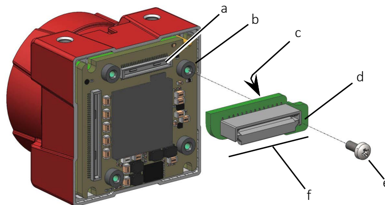
Figure 1: Alvium Flex camera, Add-on Board, and screw
