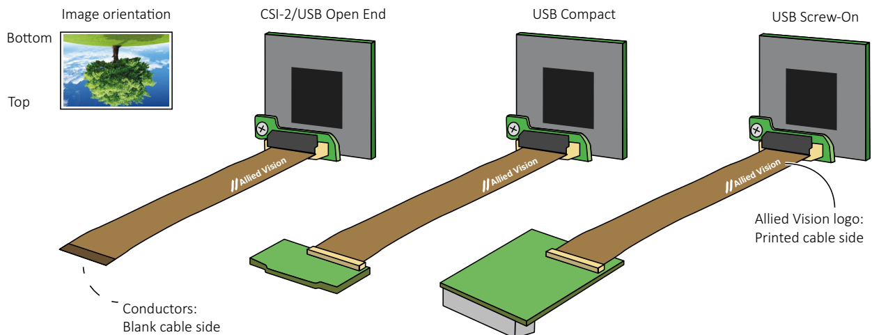
Figure 19: Alvium Flex assemblies (schematic view)
