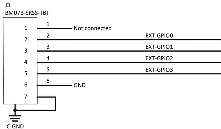
Figure 16: USB Interface Board Compact: I/O pin assignment
