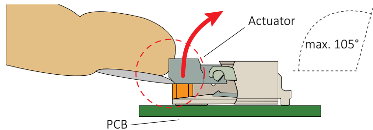
Figure 22: Opening the FPC connector
