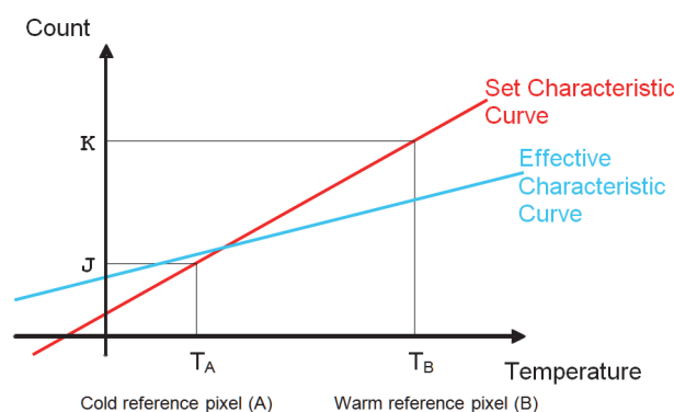
Figure 22: Two-point correction
