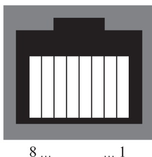
Figure 20: Front view of the Gigabit Ethernet connector
