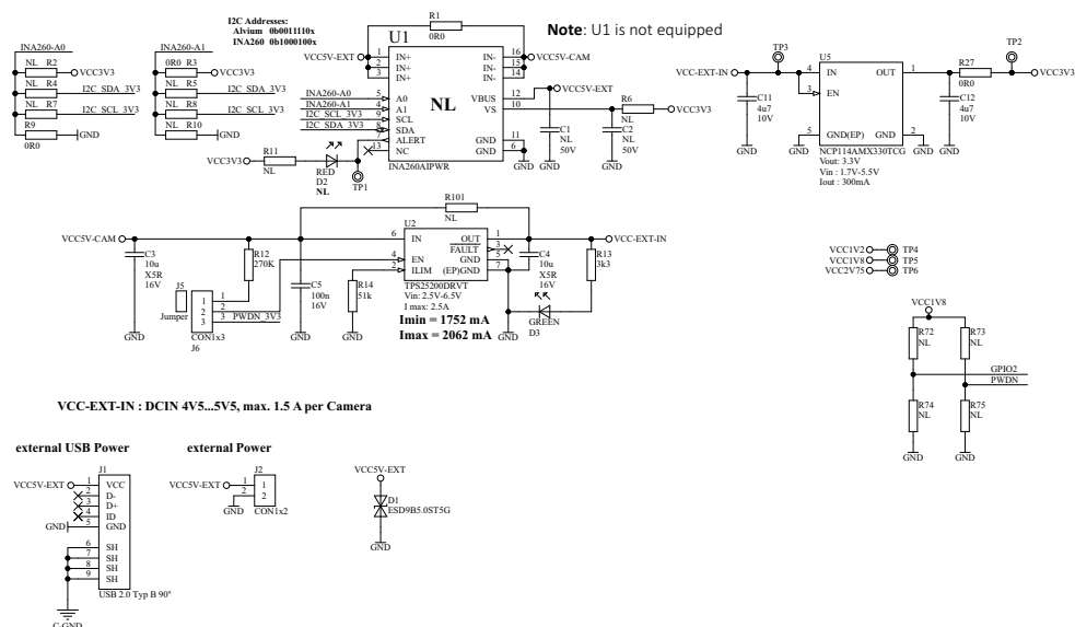
Figure 4: Adapter for Xilinx Kria KV260 electronic schematics
