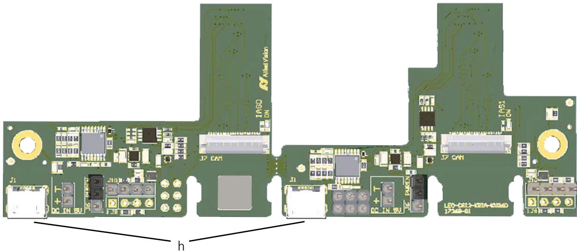
Figure 12: USB power connectors of the adapter board
