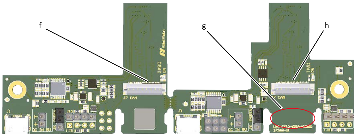
Figure 11: FPC camera connectors of the adapter board (top view)
