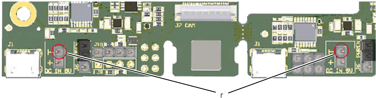
Figure 15: Ground connectors of the adapter board
