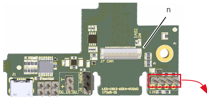
Figure 13: Camera connection to IAS1
