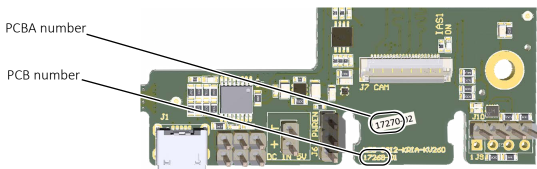
Figure 2: PCB and PCBA number on the adapter board
