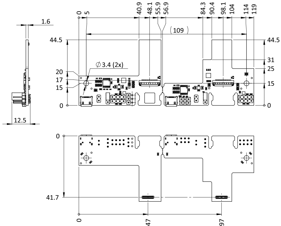
Figure 3: Adapter for Xilinx Kria KV260 dimensions and PCB layout
