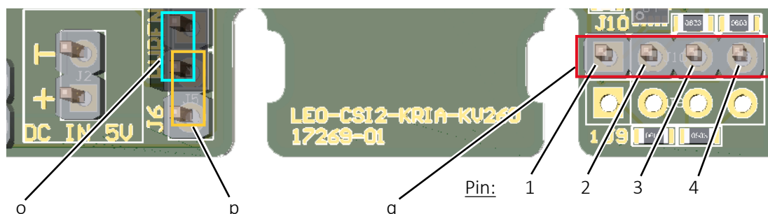
Figure 14: Connecting the I/Os for camera connection to IAS1
