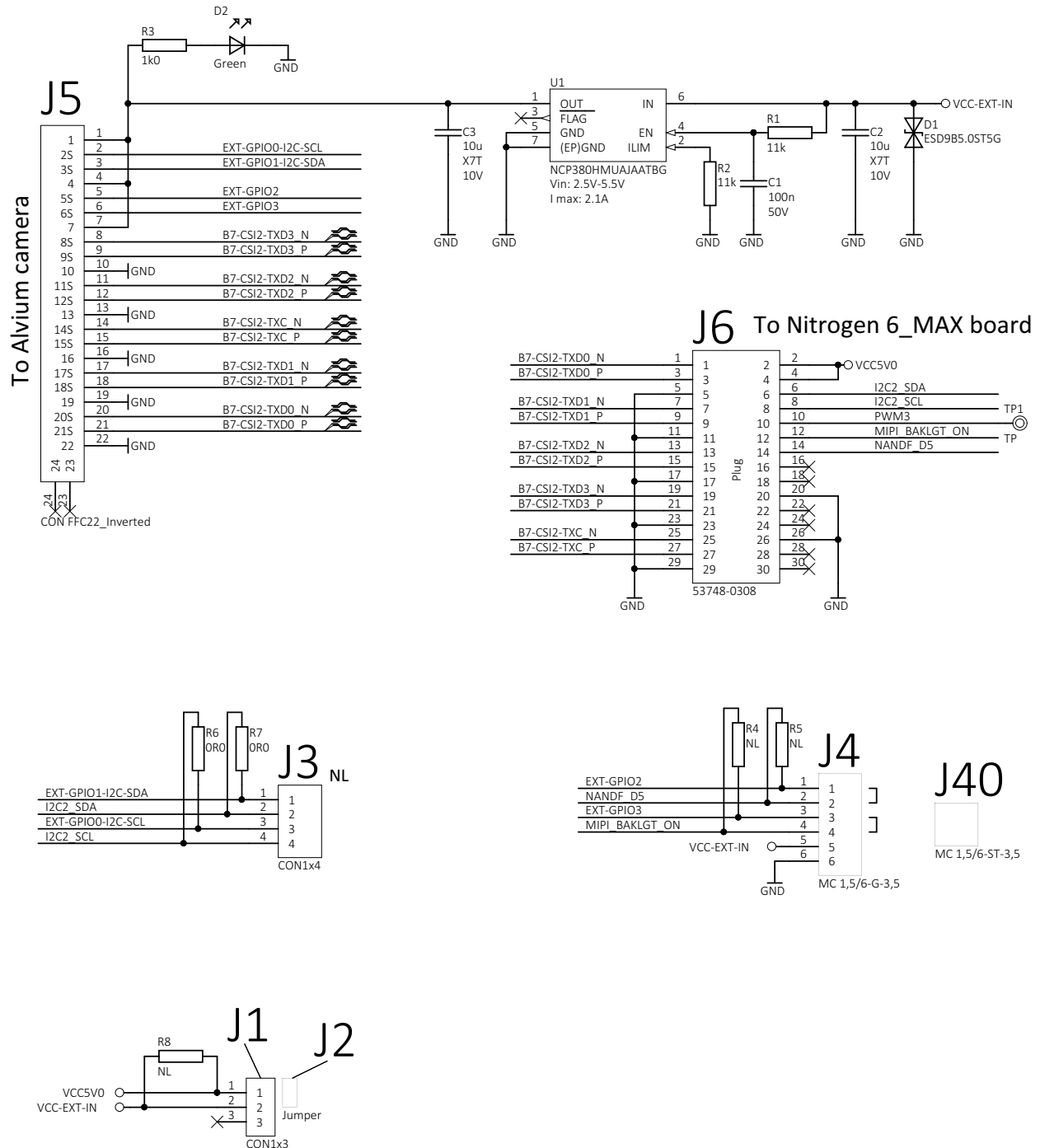
Figure 3: Adapter for Nitrogen6_MAX electronic schematics
