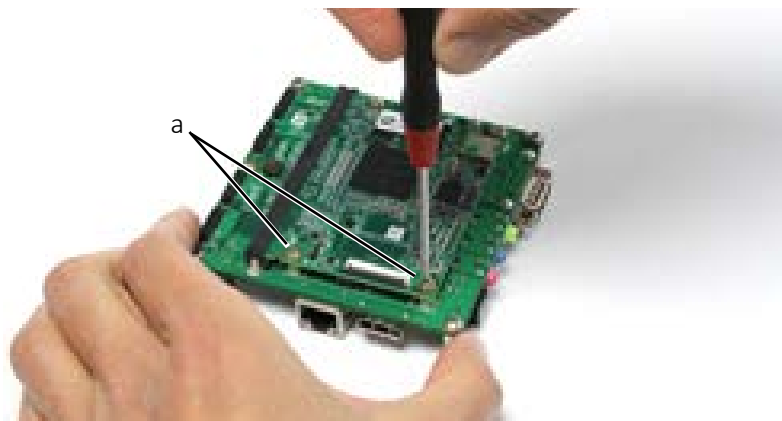
Figure 23: Removing top board bolts
