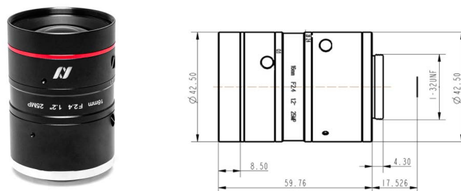
Figure 4: C-16-F2.4-25MP-T1.2- GS lens with grub type locking screws
