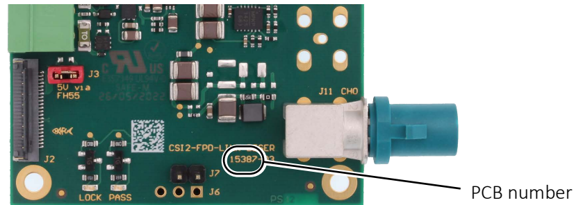
Figure 4: PCB on deserializer boards
