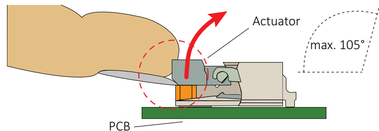
Figure 13: Opening the FPC connector
